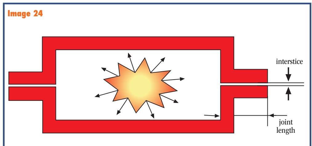
Image 24 Explosion-proof “Ex d” method of protection
