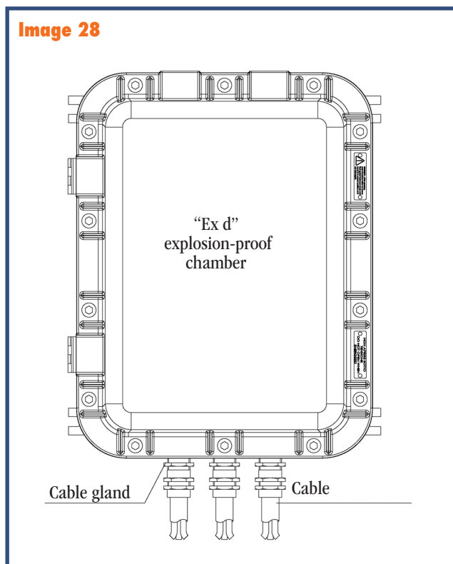
Image 28 Cable installation with direct entry
