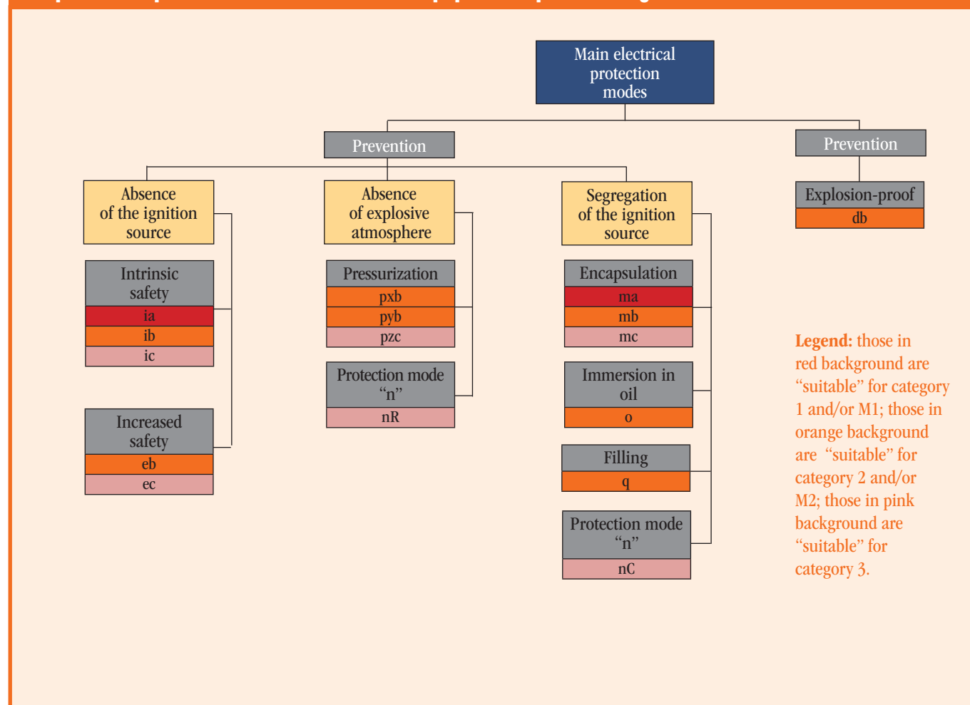
Graph 6 Main protection modes for electrical equipment in presence of gas
