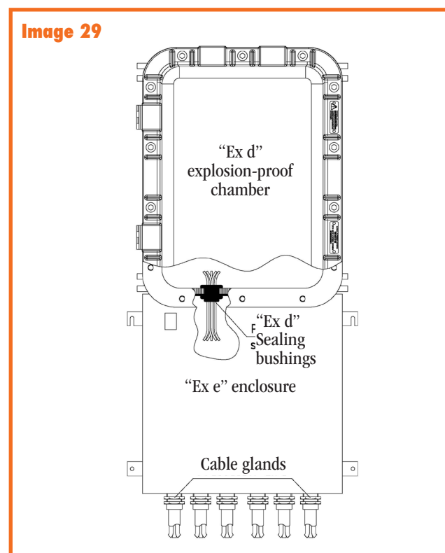
Image 29 Cable installation with indirect entry
